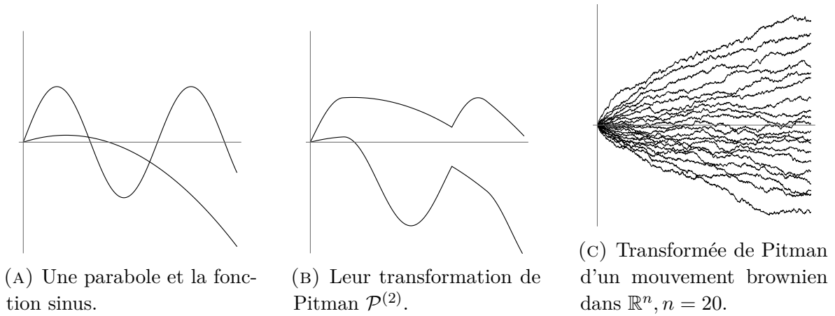
FIGURE 4. La transformation de Pitman.
